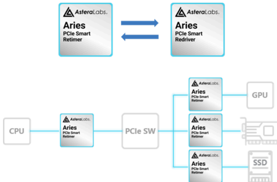
Pin Compatibility Between Smart Retimer and Redrivers for Architecture Flexibility
